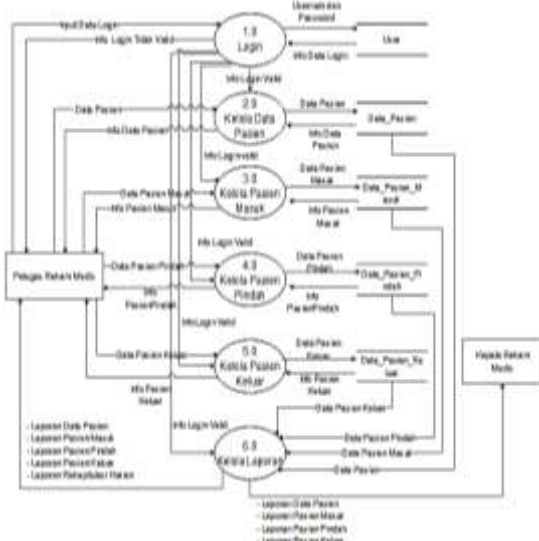
Gambar 4. DFD Level 0 Sensus Harian Rawat Inap
