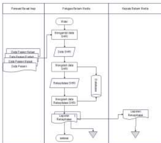
Gambar 2. Flowmap Sensus Harian Rawat Inap
