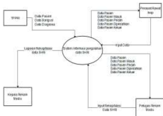
Gambar 3. Diagram Konteks Sensus Harian Rawat Inap
