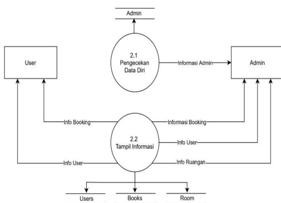
Gambar 6. DFD Level 2
