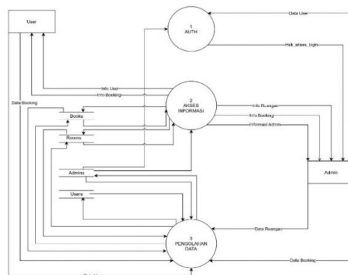
Gambar 3. DFD Level 1
