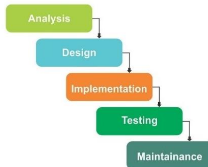
Gambar 1. Metode Waterfall
